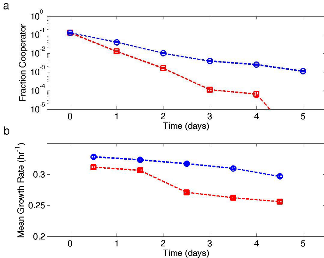
Supplementary Figure 9: Evolution of a competing culture can lead to decreasing growth rates. Two cultures in 5% sucrose and 0.03% glucose were started with an initial fraction of 13% cooperators. Over time both the 0.2X HIS (blue circle) and 0.05X HIS (red square) cultures had a decrease in the fraction of cooperators (a) and the growth rate (b). The decreasing fitness over time is a striking manifestation of the cooperative interaction, as evolutionary dynamics normally lead to an increase in the mean fitness of a population 12 .
